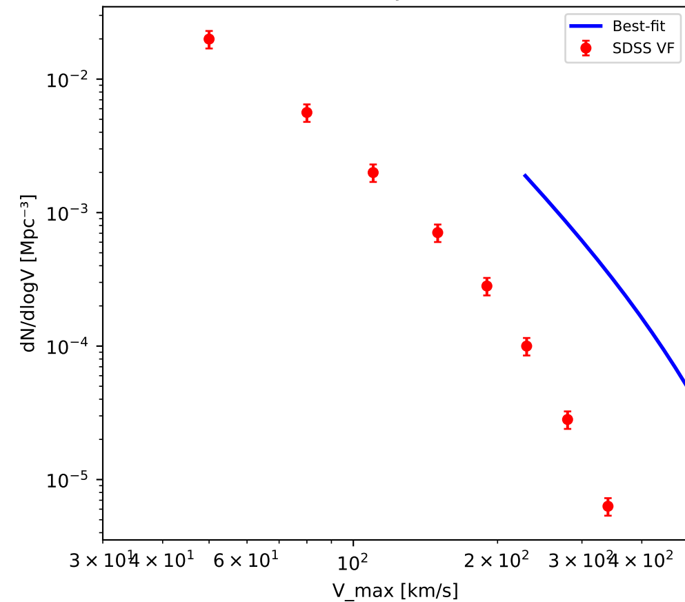
(a) Velocity Function
