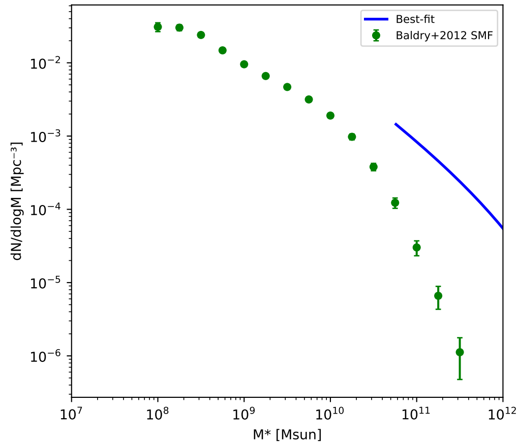
(b) Stellar Mass Function
