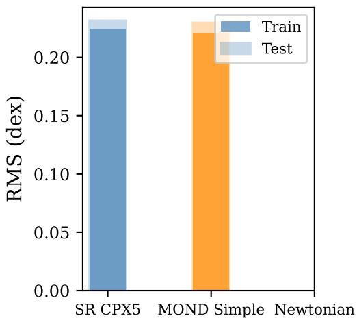
(e) Holdout (10-fold)
