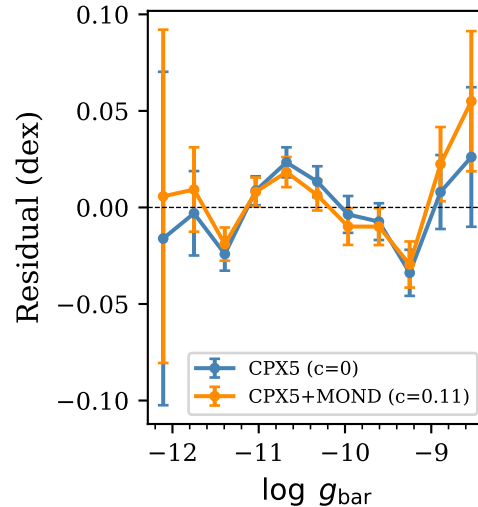
(f) MOND asymptote test: c = 0.11 \pm 0.15
