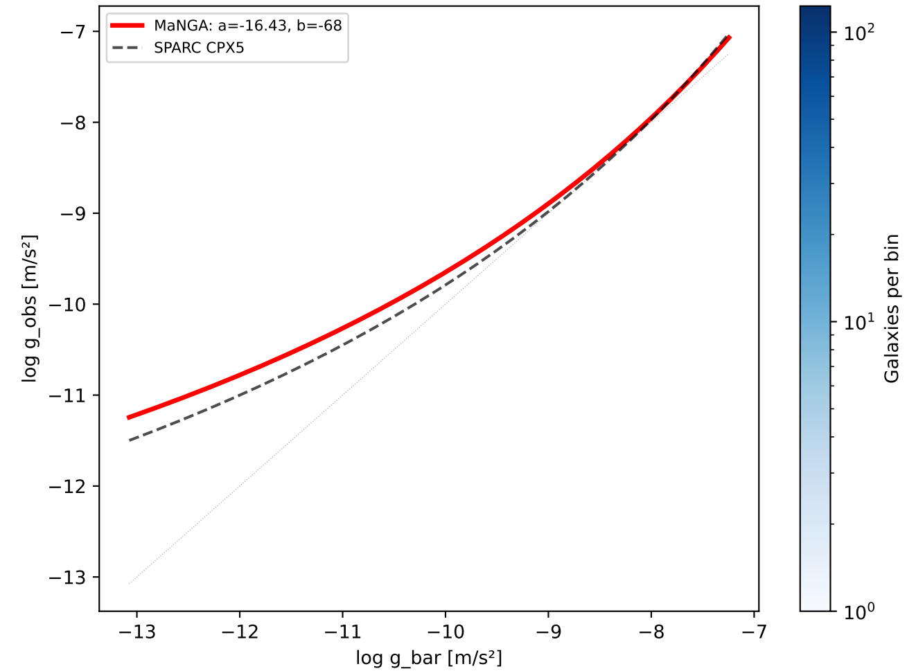
(a) MaNGA RAR (10052 galaxies)
