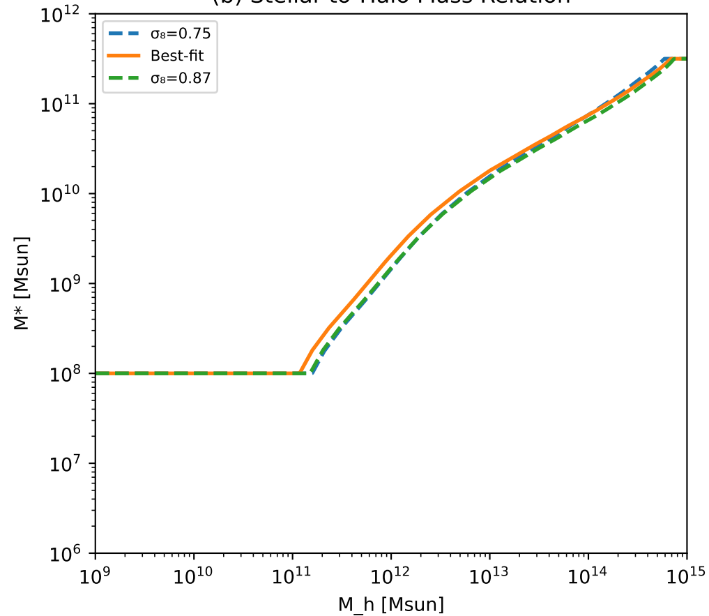
(b) Stellar-to-Halo Mass Relation
