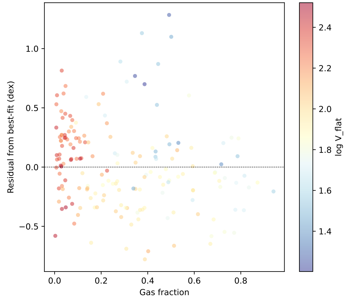
(c) Residual vs Gas Fraction ( \rho = -0.27 )
