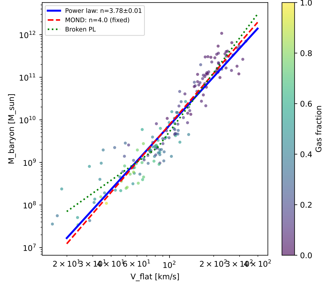
(a) Baryonic TFR (171 galaxies)
