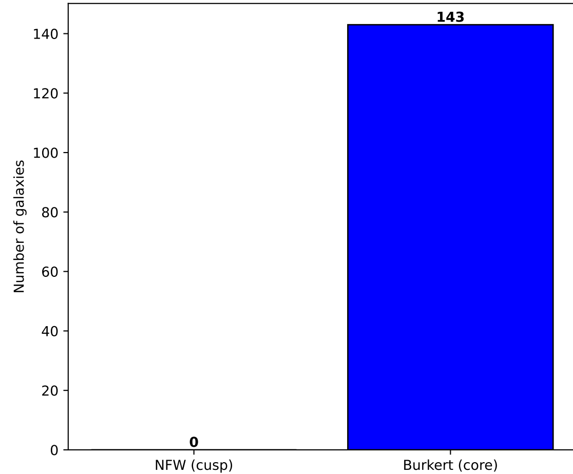
(c) Preferred Model ( \Delta AIC , 143 galaxies)
