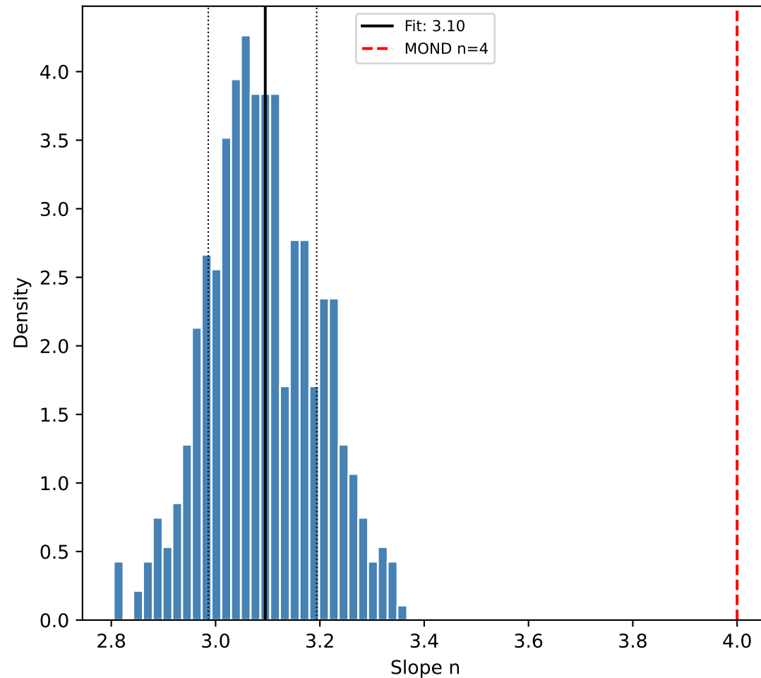
(b) Bootstrap: n=3.09 \pm 0.10 ( 8.7\sigma from MOND)
