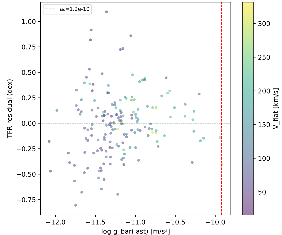
(c) Residual vs g_{\text{bar}} ( \rho=0.14 )
