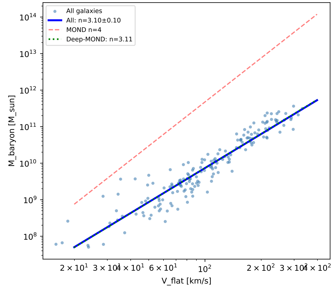
(a) Baryonic TFR (171 galaxies, RMS=0.309 dex)
