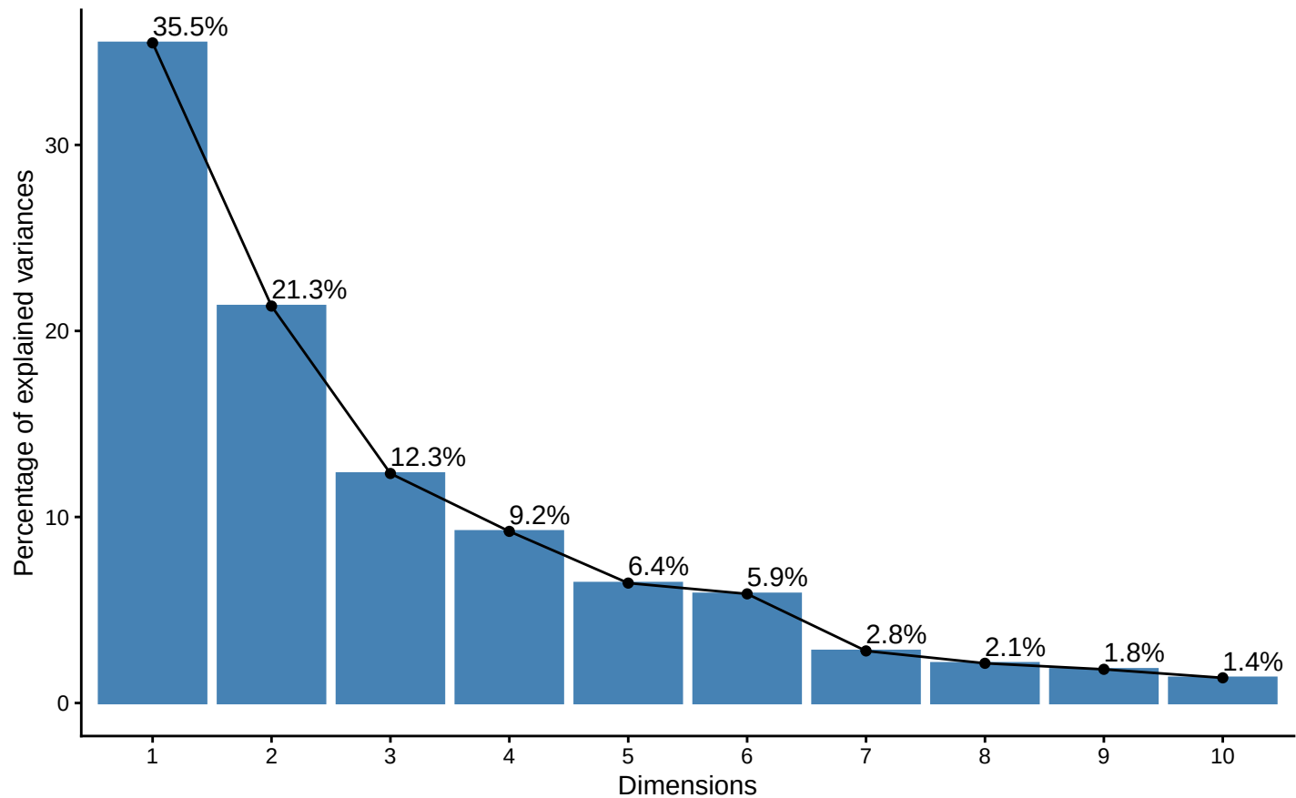
Scree plot
