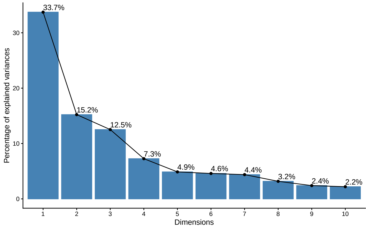
Scree plot
