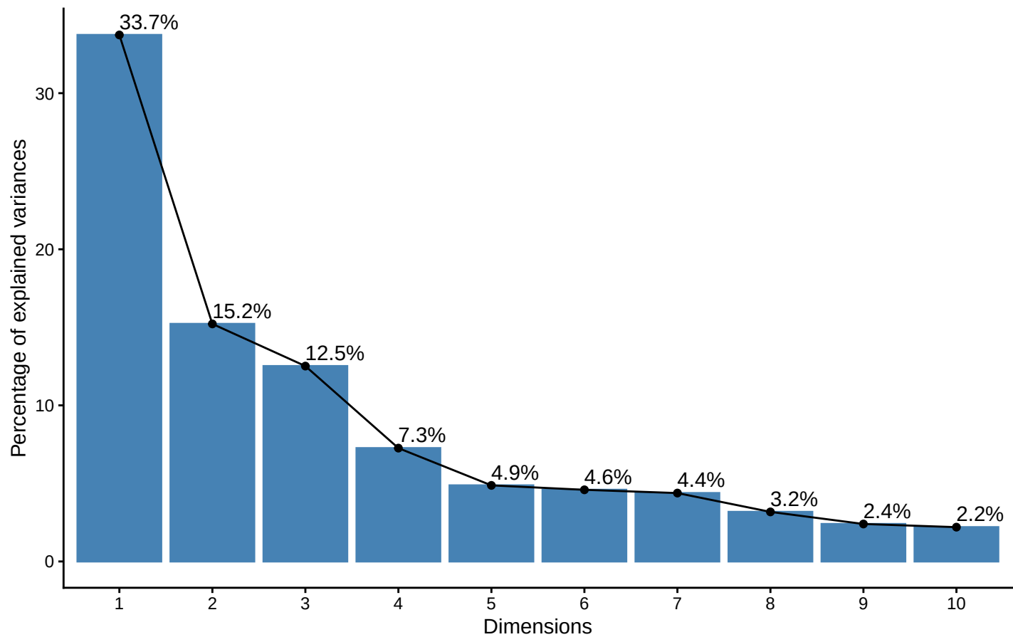
Scree plot
