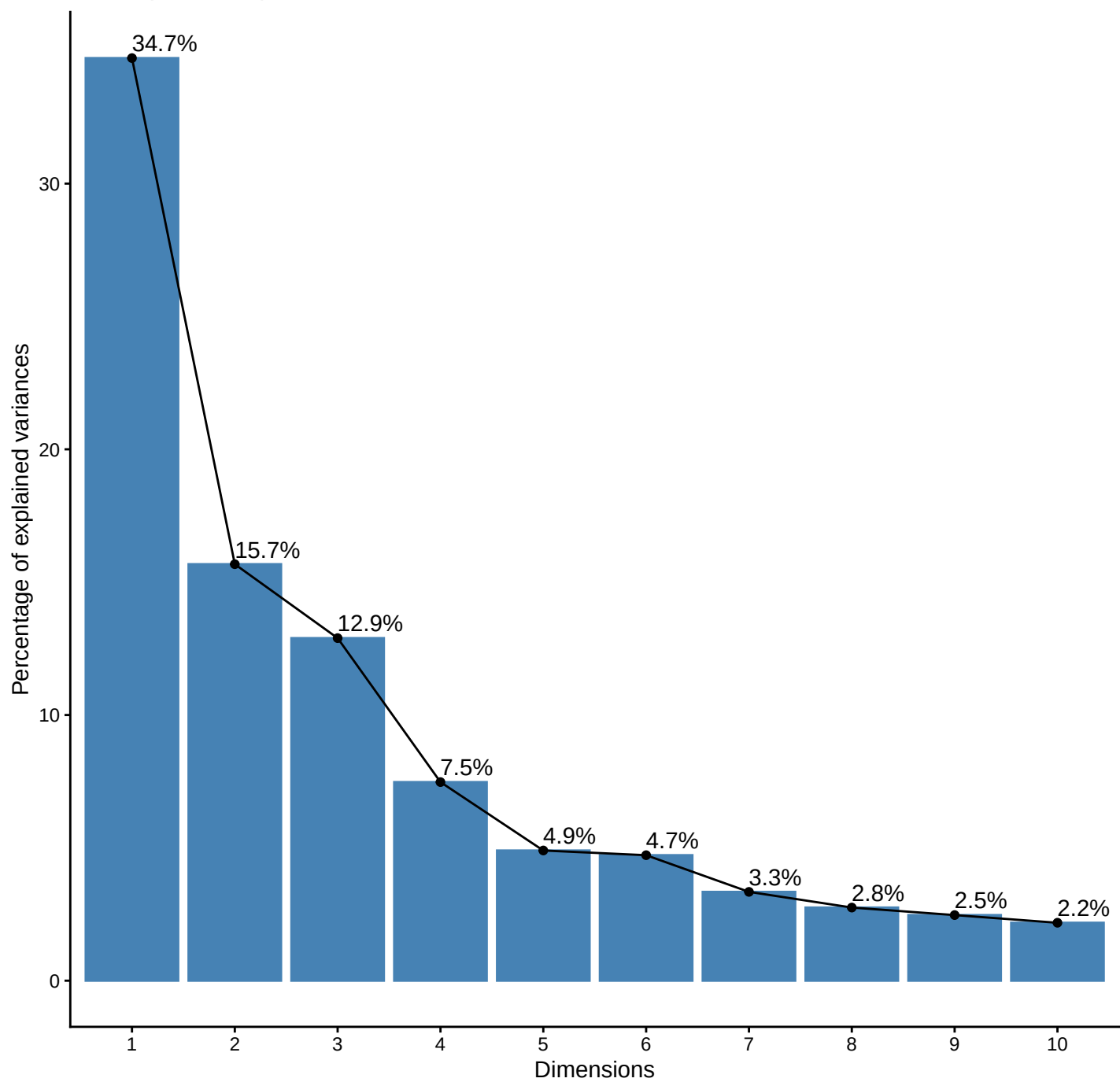
Scree plot – all parameters
