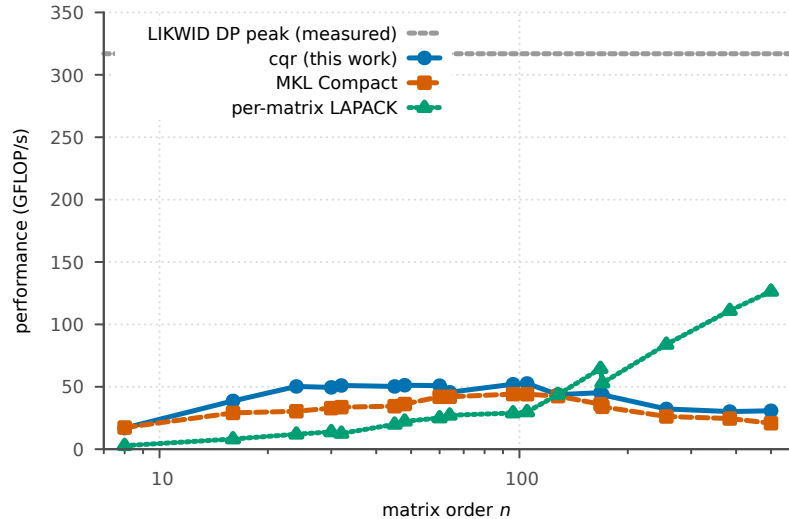
QR factorisation rate on x86 (AVX-512) vs LIKWID roofline
