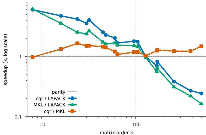
Speedup over per-matrix LAPACK (x86, AVX-512)
