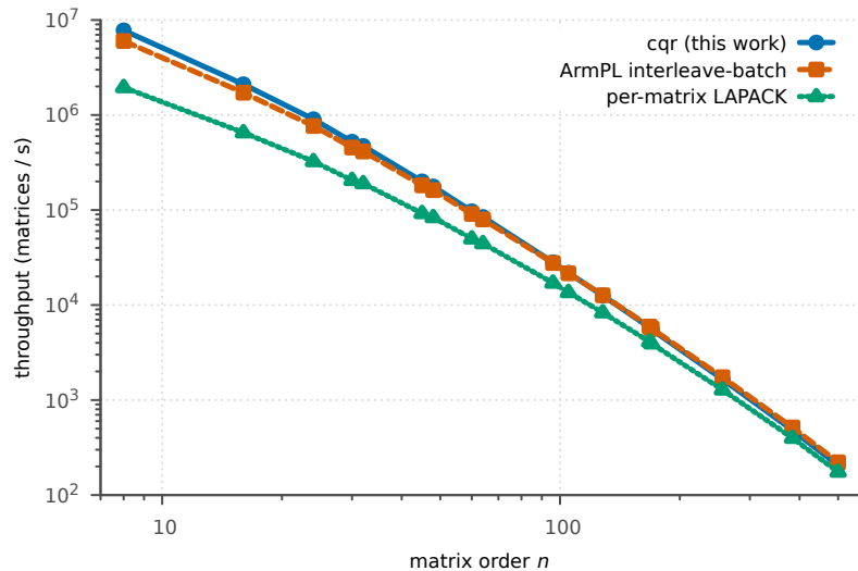
QR factorisation throughput on Arm (SVE)
