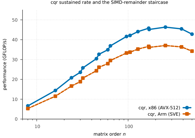
Figure 5: cqr sustained rate (GFLOP/s) vs order on x86 and Arm. The wiggle at non-multiple-of- V orders is the SIMD-remainder staircase. Placeholder data.
