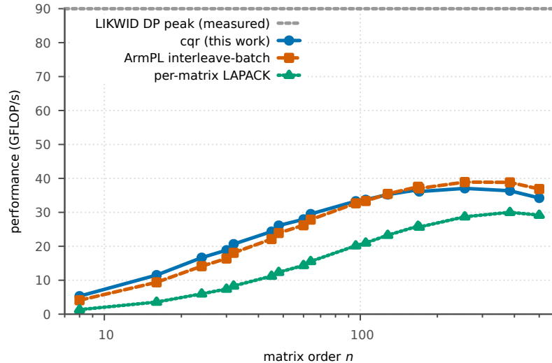
QR factorisation rate on Arm (SVE) vs LIKWID roofline
