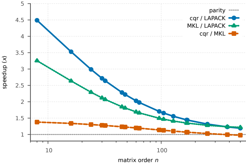
Speedup over per-matrix LAPACK (x86, AVX-512)
