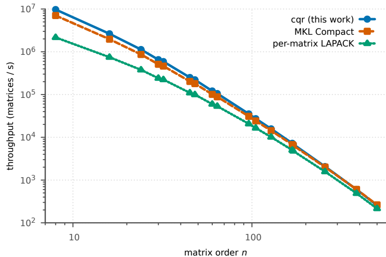
QR factorisation throughput on x86 (AVX-512)
