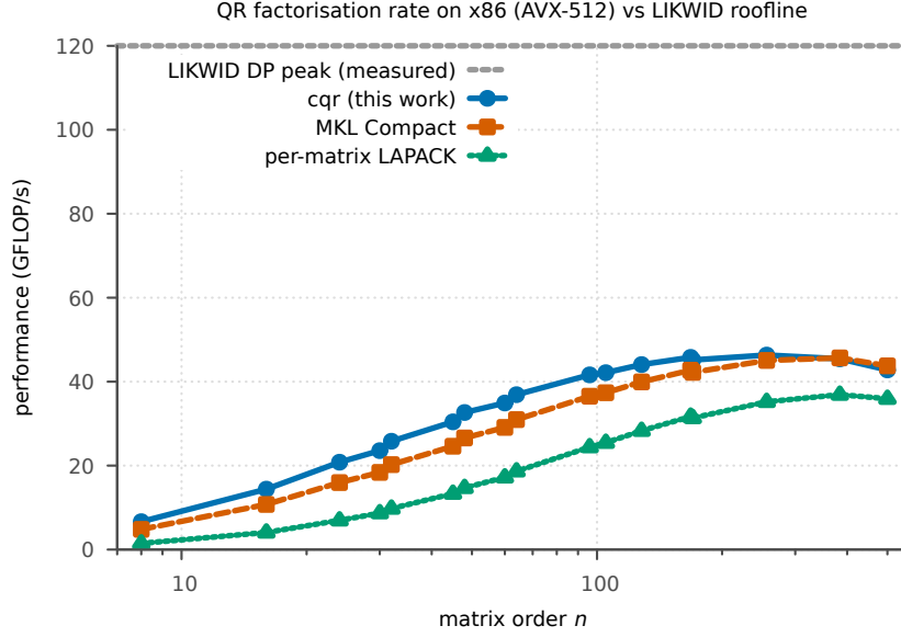
Figure 5: Achieved rate (GFLOP/s) of cqr , MKL Compact, and per-matrix LAPACK on x86 (AVX-512), against the LIKWID-measured double-precision peak. Placeholder data; placeholder roofline.
