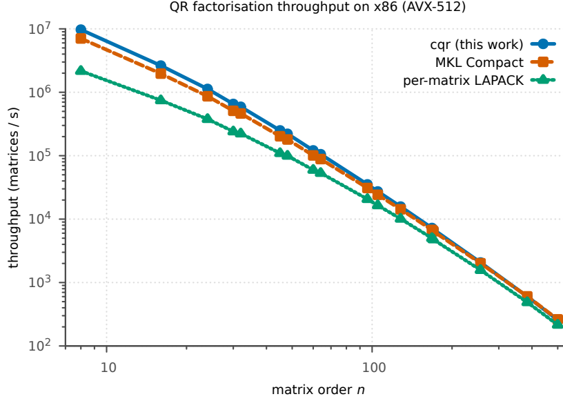
Figure 2: Batched QR factorization throughput on x86 (AVX-512): cqr vs MKL Compact vs a per-matrix LAPACK loop, over the target size range. Placeholder data.
