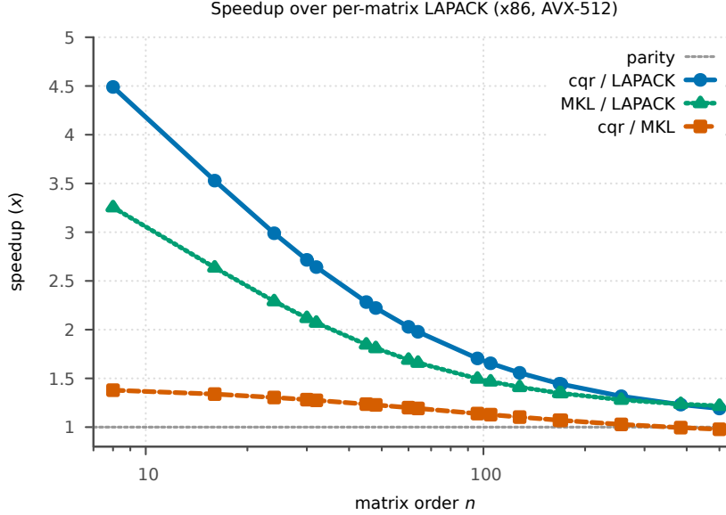
Figure 3: Speedup over the per-matrix LAPACK baseline on x86. The batched advantage is largest at the smallest orders and narrows toward the parity line as n grows. Placeholder data.
