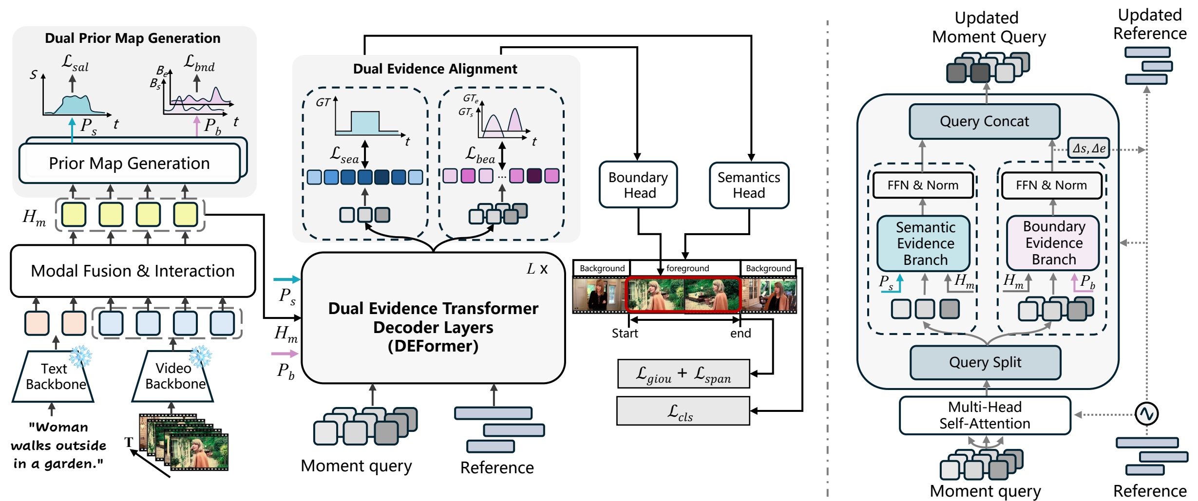
(a) Overall framework of DE 2 TR
