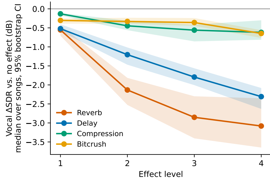
Demucs (htdemucs)
