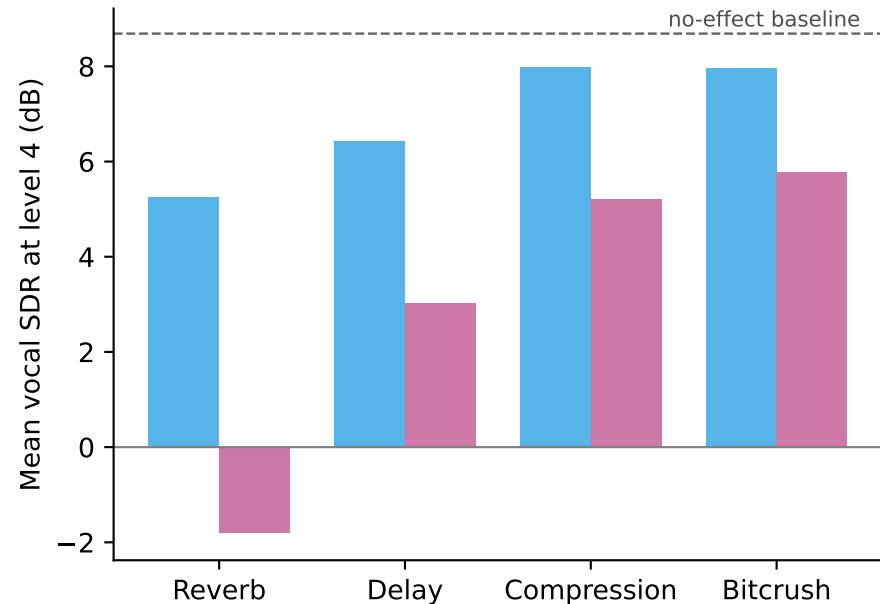
Demucs (htdemucs)
