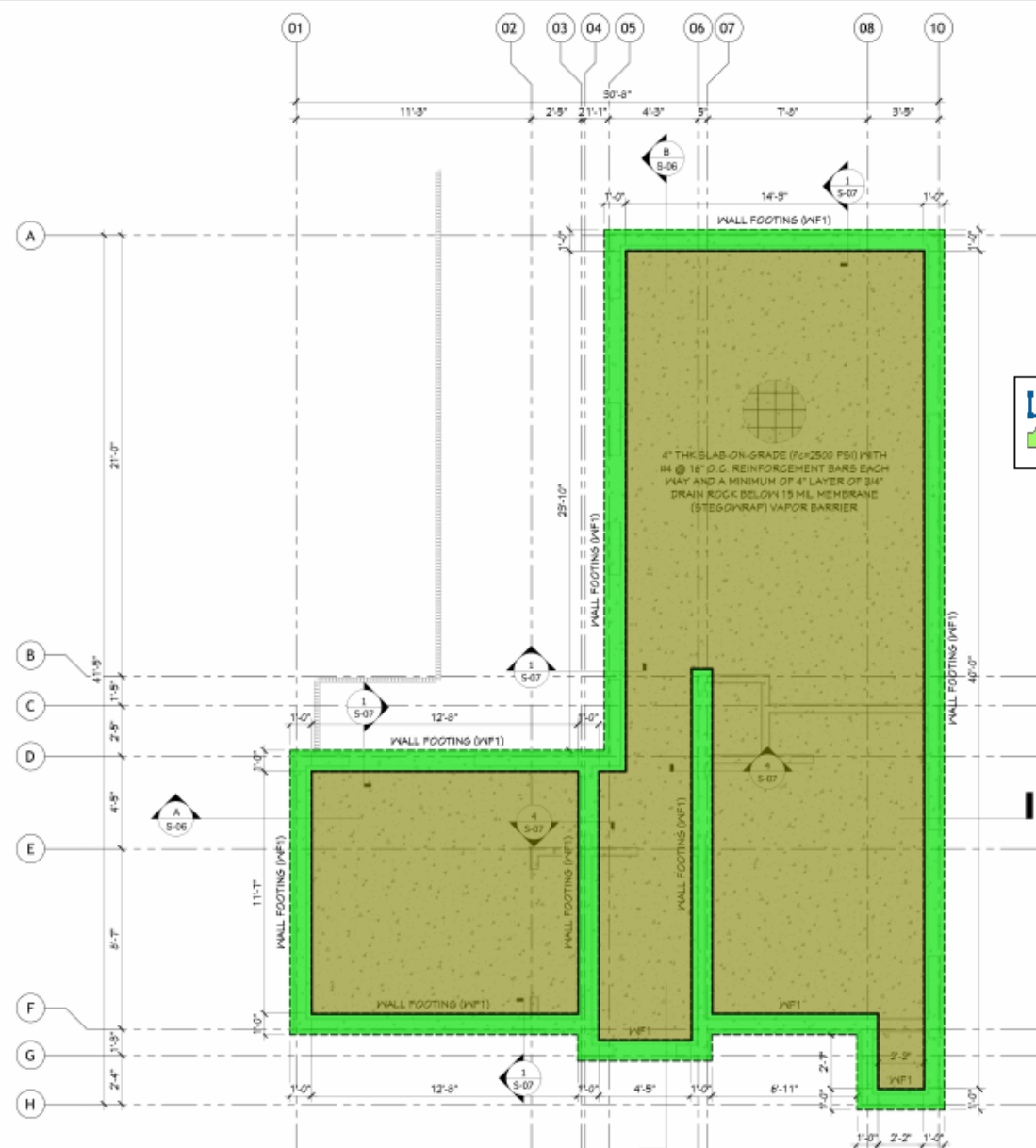
PROPOSED FOUNDATION PLAN SCALE 3/8" = 1'-0"
