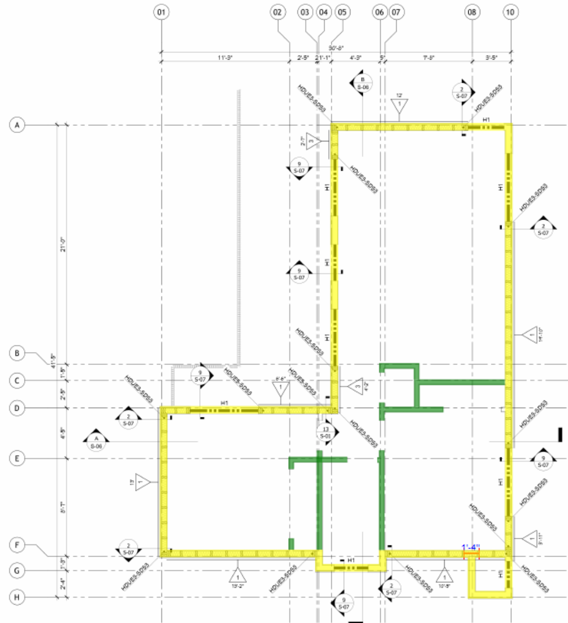
PROPOSED SHEARWALL LAYOUT PLAN SCALE 3/8" = 1'-0"
