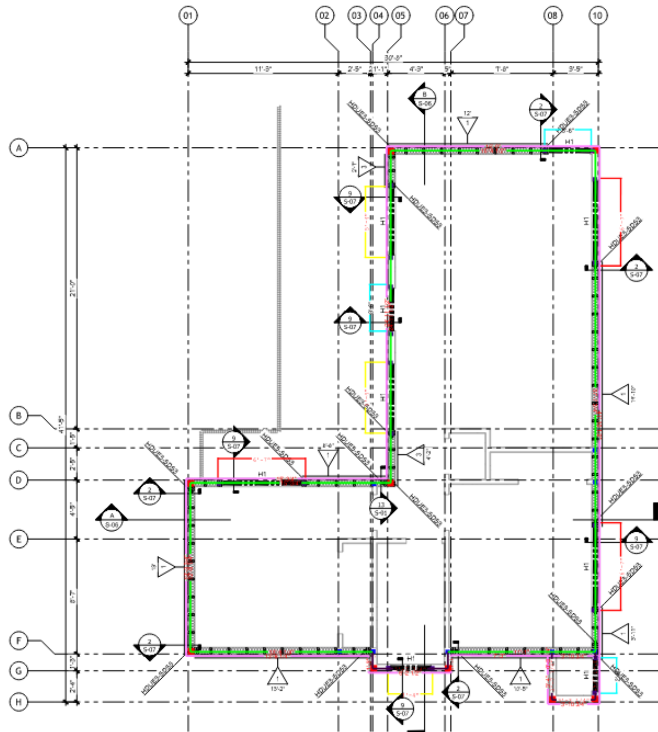
PROPOSED SHEARWALL LAYOUT PLAN
