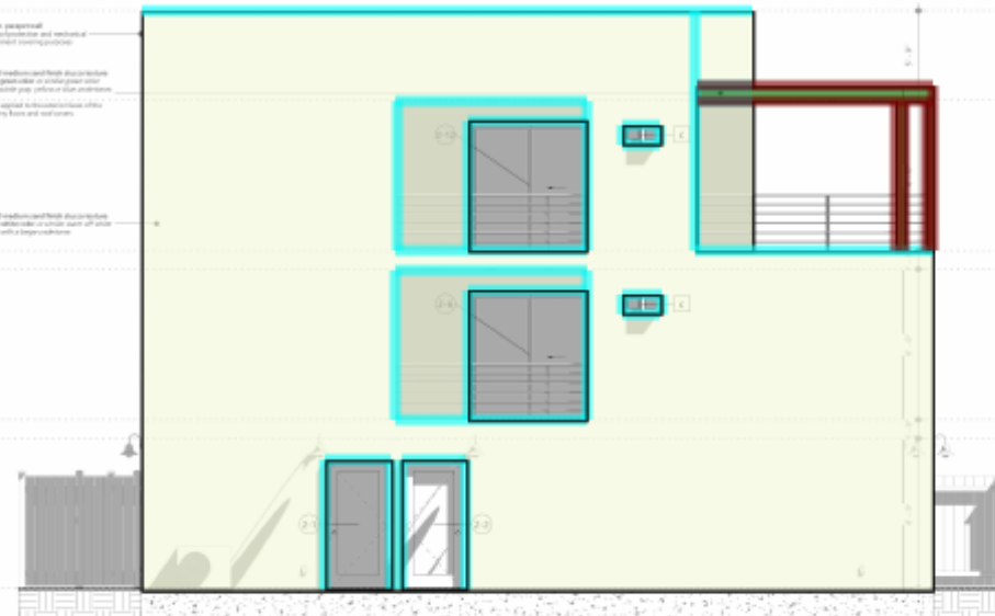
SOUTH PROPOSED | ACCESSORY DWELLING UNIT
