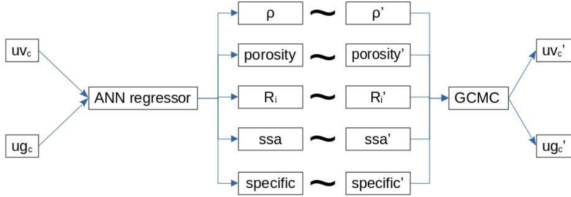
Fig. 3. ANN output as starting point to search a MOFs solution
