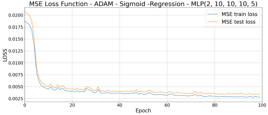
Fig. 2. MSE evolution of MLP-Regressor
