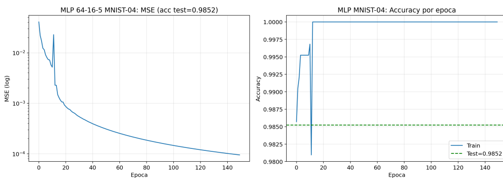
Figura 12: MLP 64–16–5 en MNIST dígitos 0–4 (98.5 % test).
