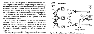
Fig. 16. Typical two-layer Madaline II architecture.
