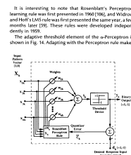
Fig. 14. The adaptive threshold element of the Perceptron.
