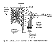
Fig. 15. A five-Adaline example of the Madaline I architecture.
