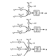
Fig. 10. Fixed-weight Adaline implementations of AND, OR, and MAJ logic functions.
