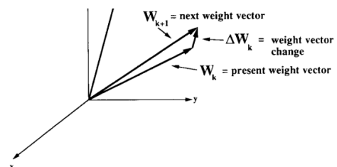
Figure 12: Fig. 12. Weight correction by the LMS rule.
