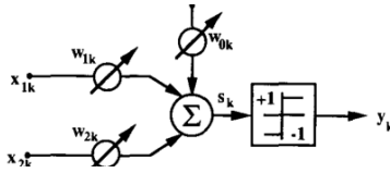
Figure 3: Fig. 3. Two-input Adaline.
