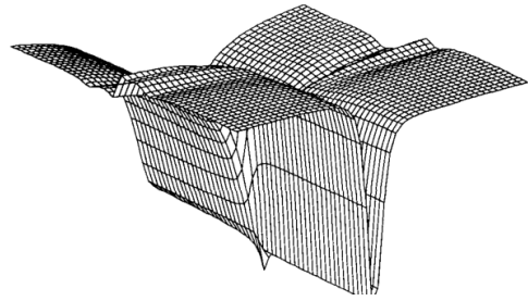
Figure 31: Fig. 32. Example MSE surface of trained sigmoidal network as a function of a first-layer weight and a third-layer weight.
