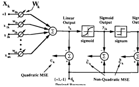
Figure 21: Fig. 21. The linear, sigmoid, and signum errors of the Ada- line.
