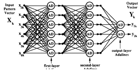
Figure 11: Fig. 11. Three-layer adaptive neural network.
