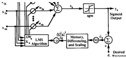
Figure 20: Fig. 20. Implementation of the MRlll algorithm for the sigmoid Adaline element.
