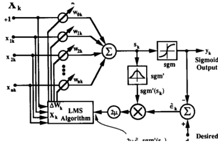
Figure 19: Fig. 19. Implementation of backpropagation for the sigmoid Adaline element.
