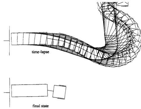
Figure 27: Fig. 27. Example truck backup sequence.
