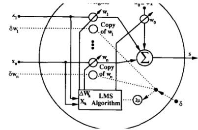
Figure 26: Fig. 26. Detail of linear combiner and associated circuitry in backpropagation network.
