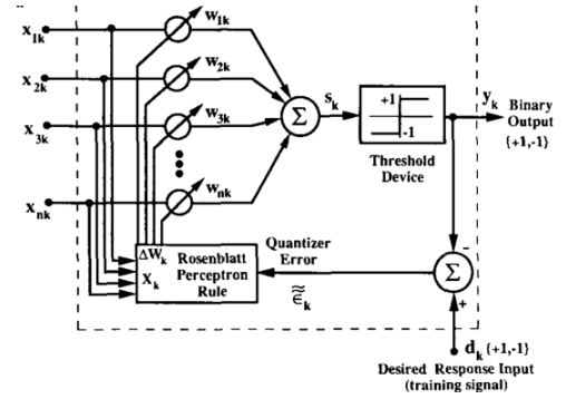
Figure 14: Fig. 14. The adaptive threshold element of the Perceptron.
