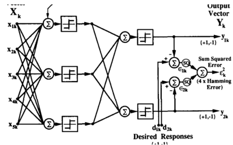
Figure 16: Fig. 16. Typical two-layer Madaline II architecture.
