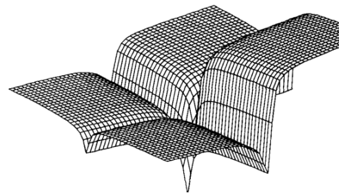
Figure 32: Fig. 30. Example MSE surface of trained sigmoidal network as a function of two first-layer weights.
