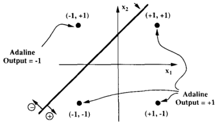
Figure 4: Fig. 4. Separating line in pattern space.
