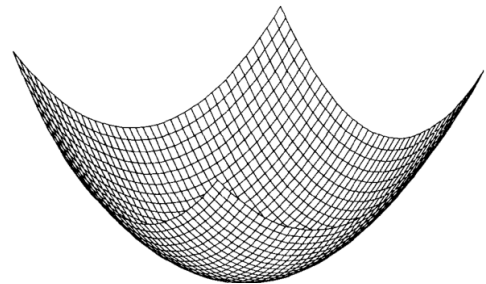
Figure 17: Fig. 17. Typical mean-square-error surface of a linear combiner.
