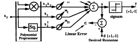
Figure 6: Fig. 6. Adaline with inputs mapped through nonlinearities.
