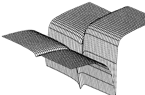
Figure 30: Fig. 29. Example MSE surface of untrained sigmoidal network as a function of two first-layer weights.
