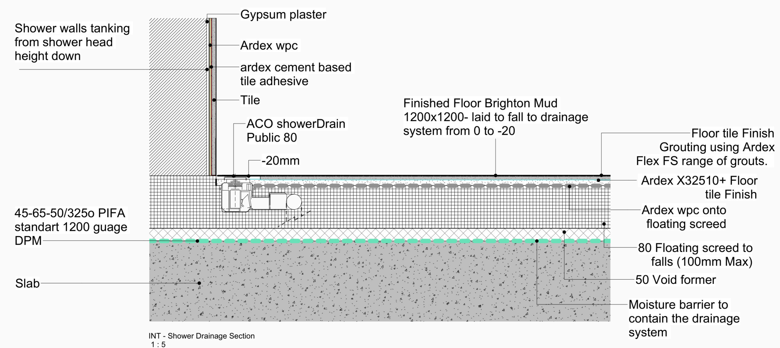
Drainage system in showers
