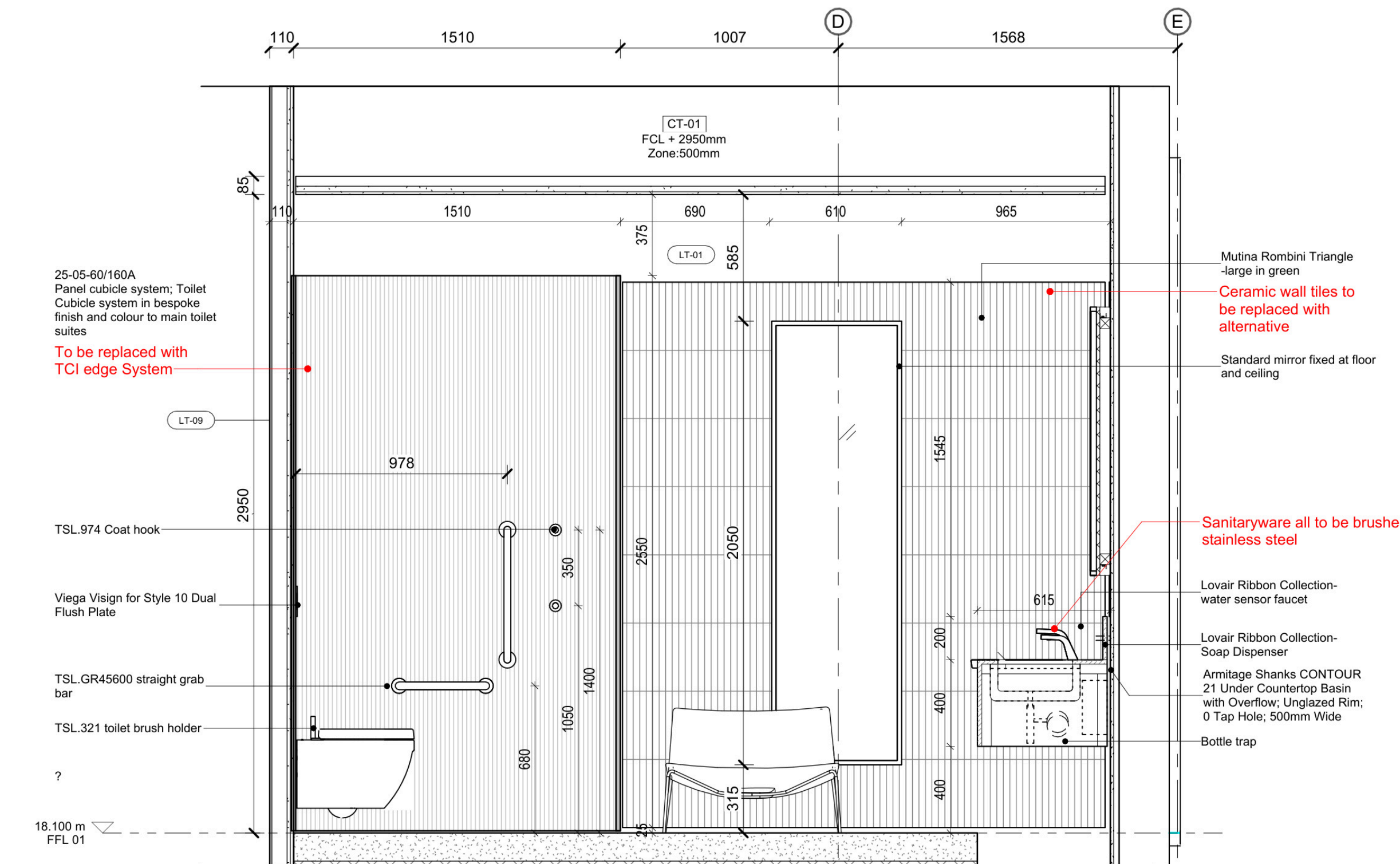
5 Female WC Elevati 1 : 20
