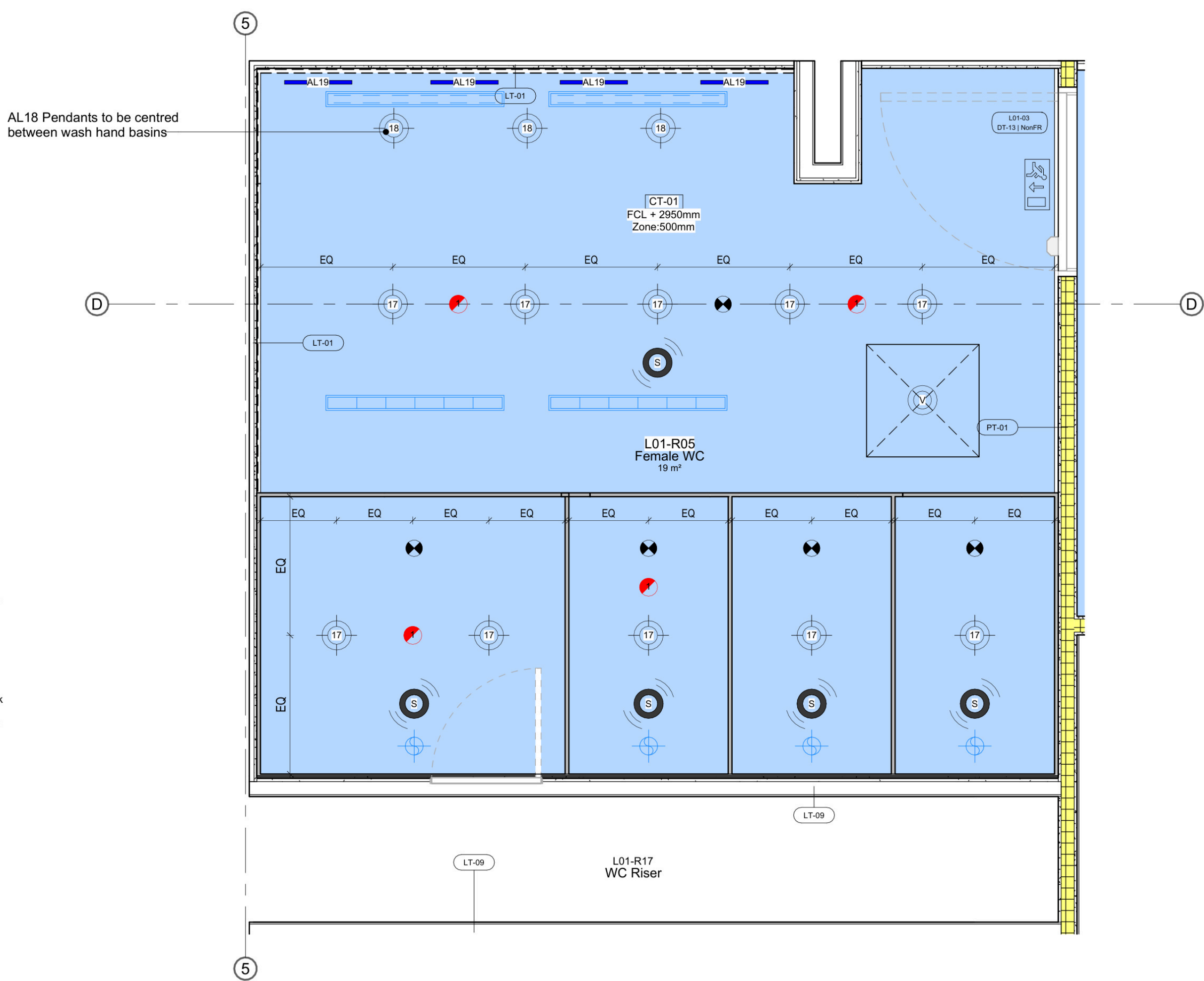
2 Female WC RCP 1 : 20
