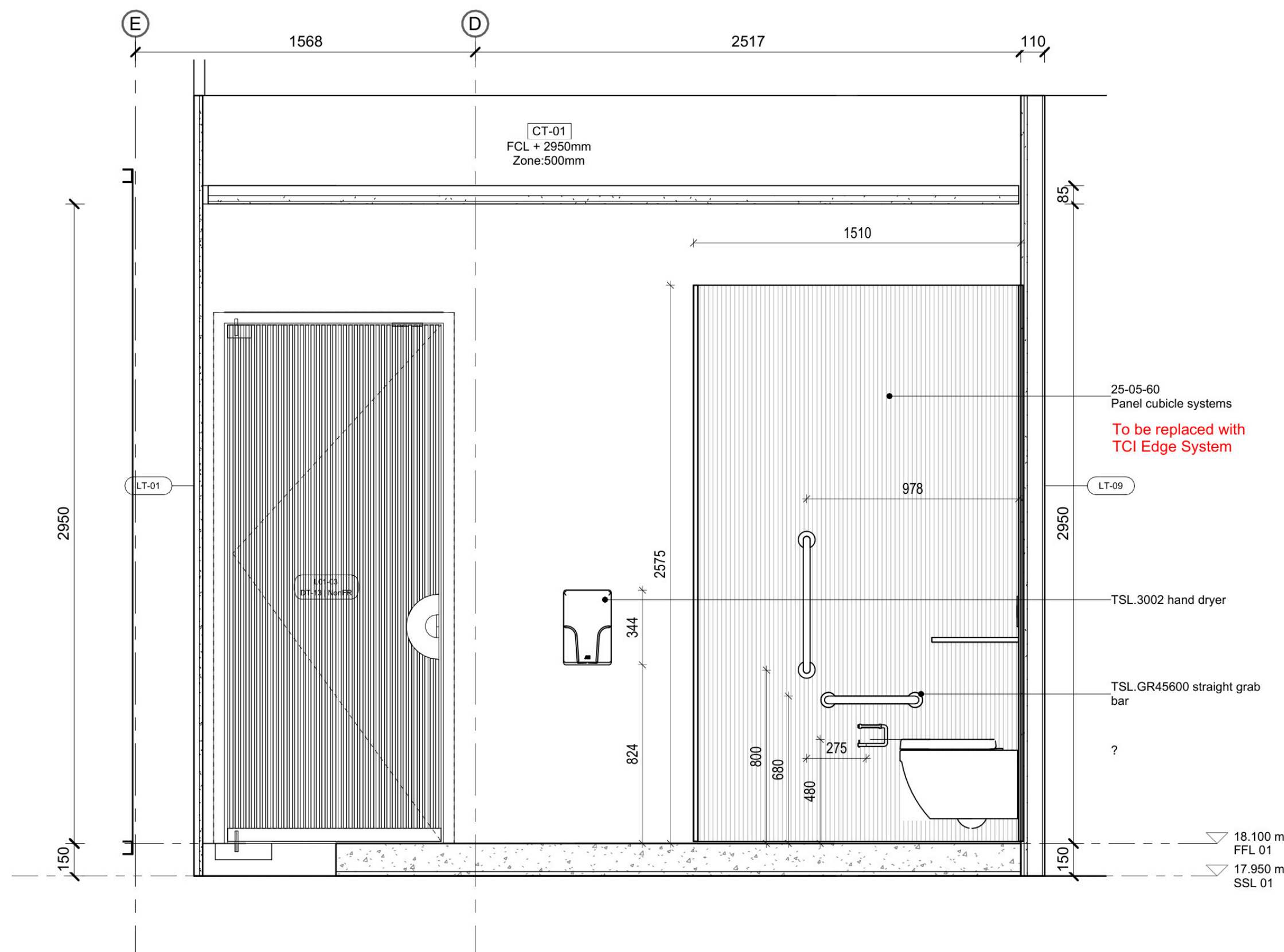
5 Female WC Elevati 1 : 20
