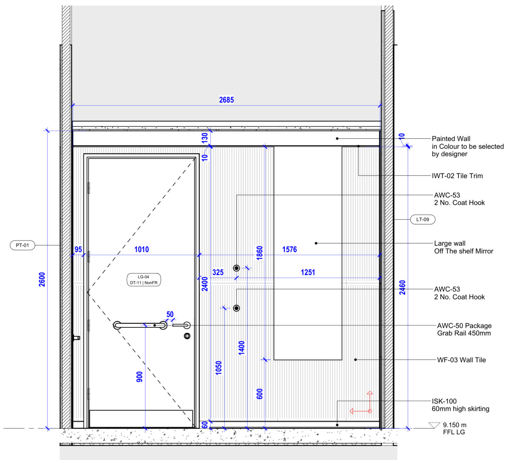
Male WC Elevation -b2 1 : 20
