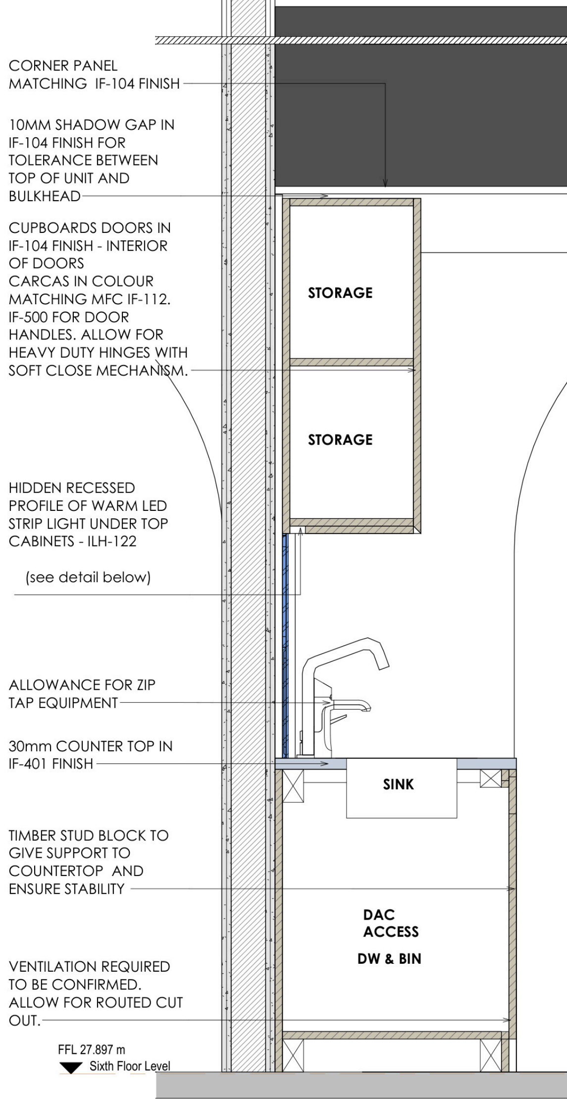
5 L06-Typical Floor Section Tea Station 6th floor 1 : 10
