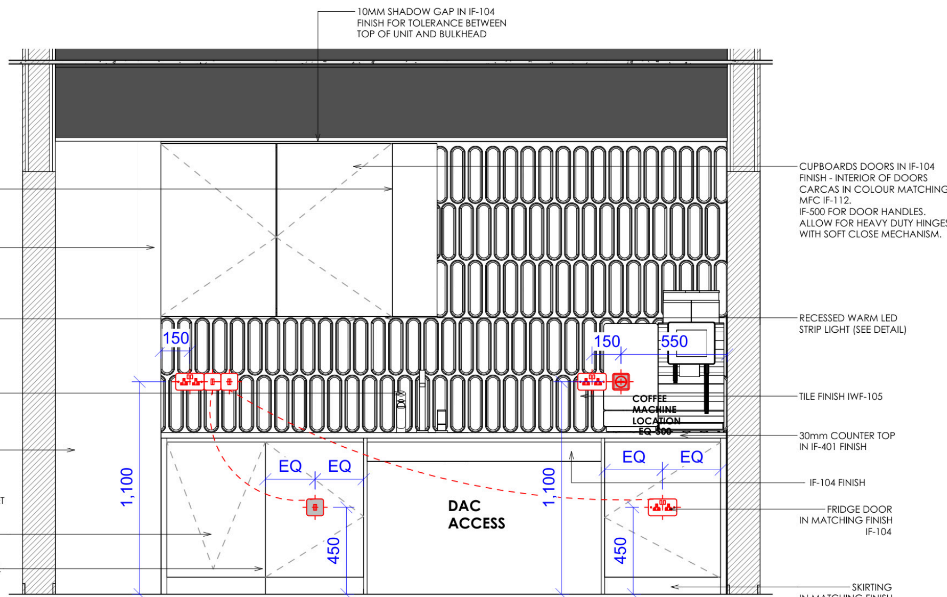
4 L06-Typical Floor Front Elevation Tea Station 6th floor 1 : 20
