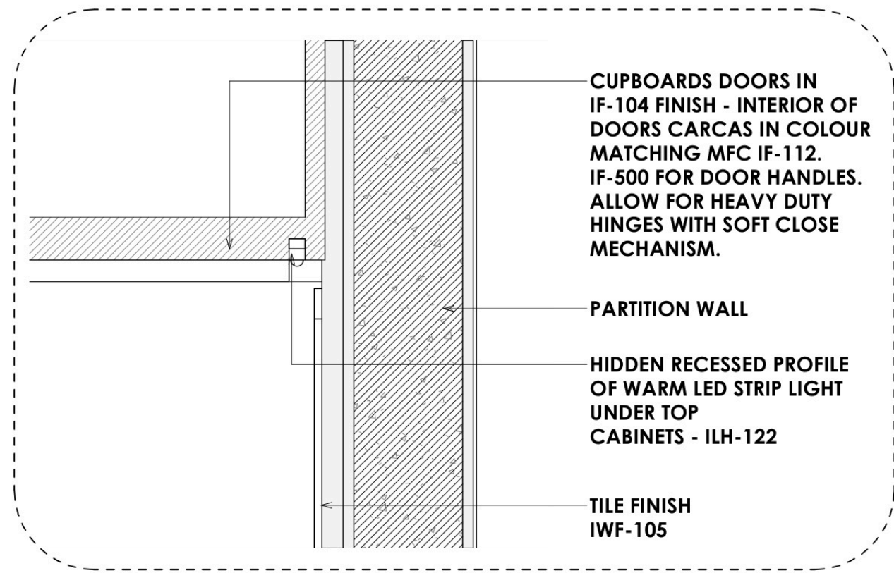
3 L06-Typical Floor Tea Station 6th Floor 1 : 5
