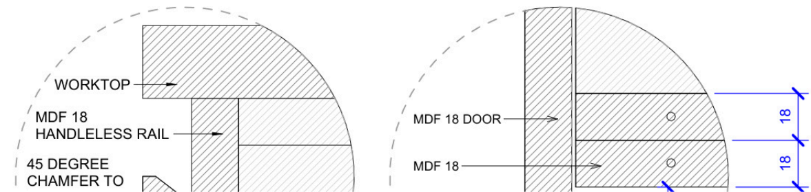
3 L06-Typical Floor Tea Station 6th Floor 1 : 5
