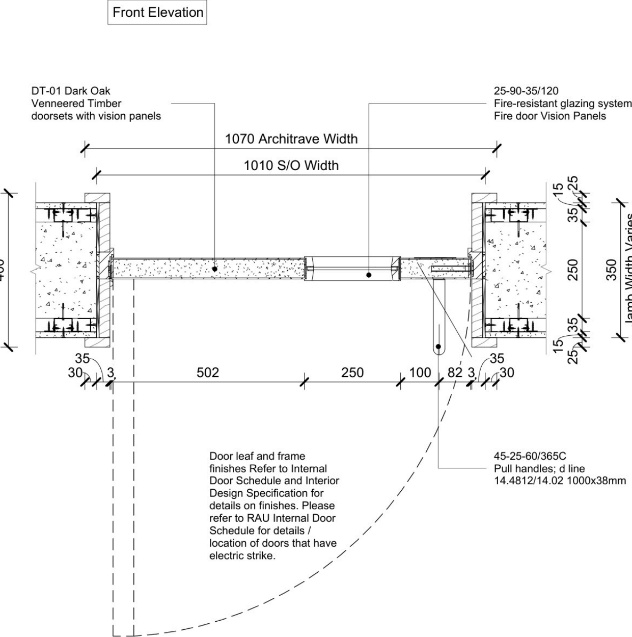
Front Elevation
