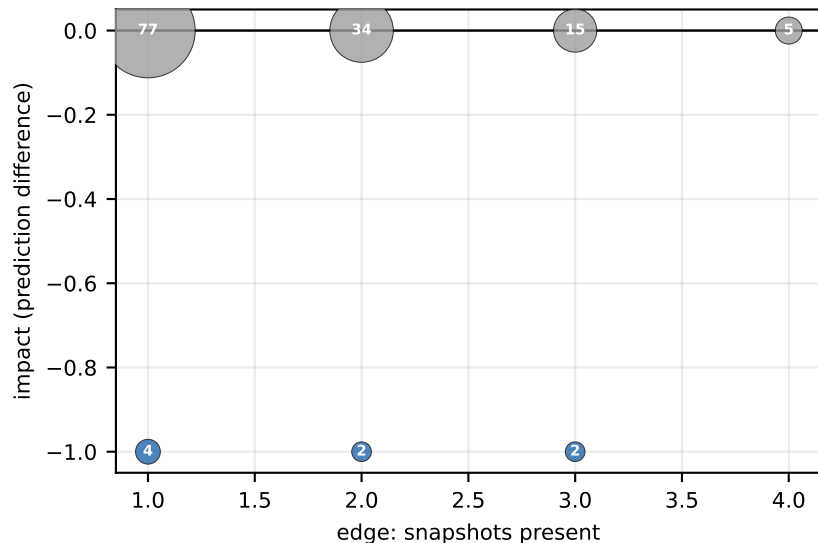
synthetic_3community - edge occlusion n=139, coverage=100%, model=PersistenceTemporalModel
