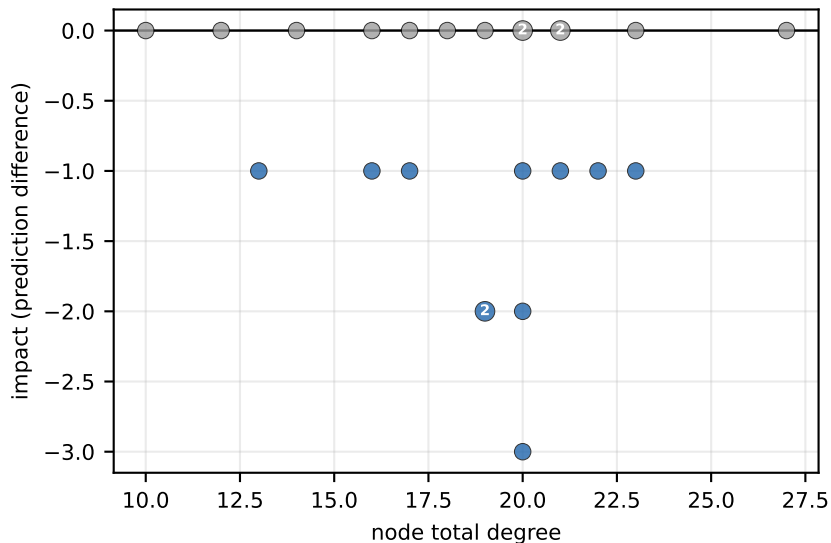
synthetic_3community - node occlusion n=24, coverage=100%, model=PersistenceTemporalModel
