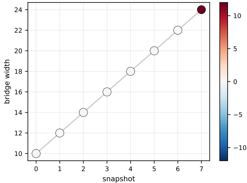
Present-only model
