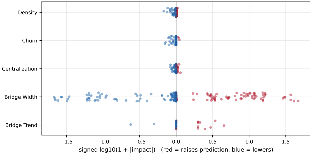
Impact distribution per concept, 8 datasets, valid rows only
