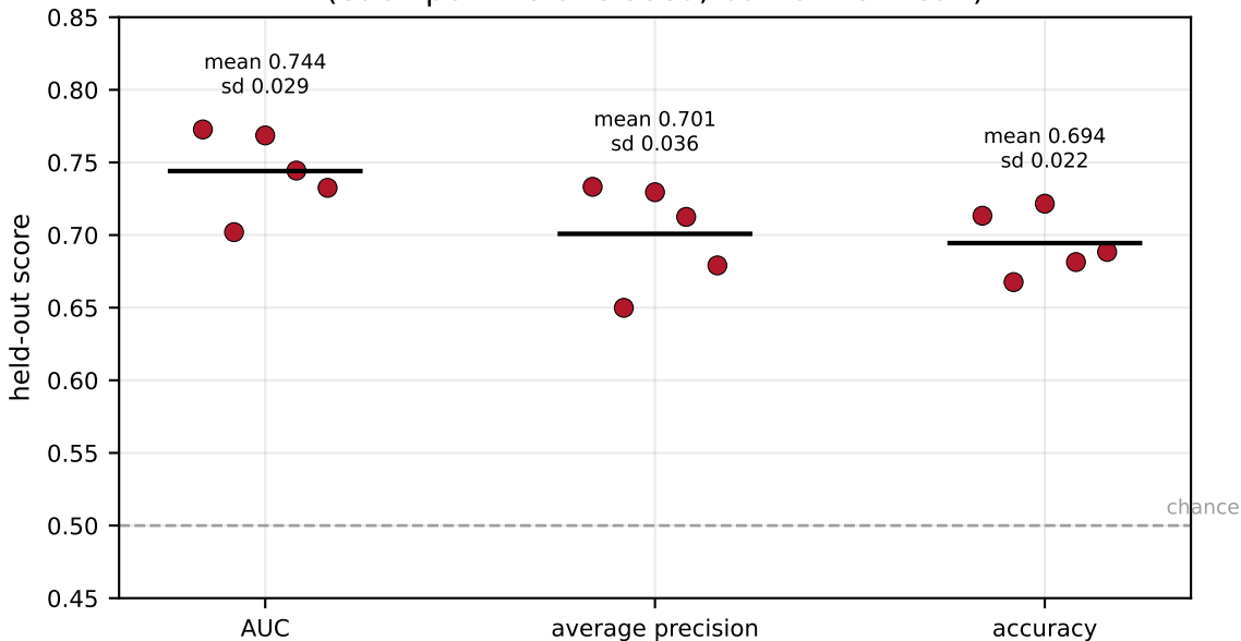
TGN held-out performance across 5 fixed seeds (each point is one seed; bar is the mean)
