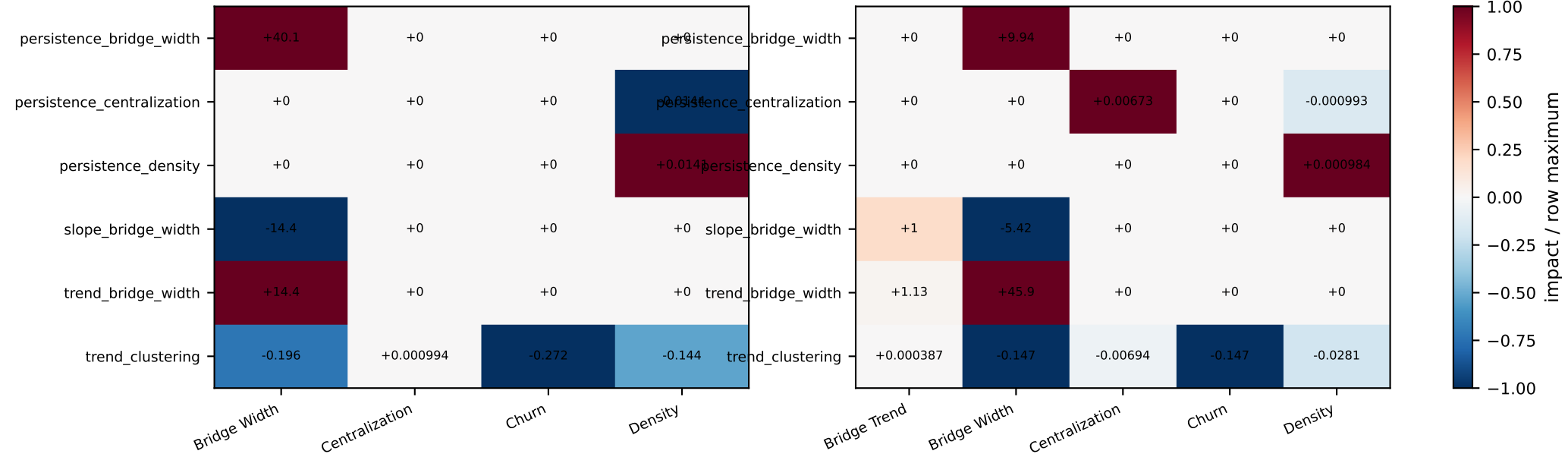
Model x concept explanation matrix (delta 0.1, increase)
