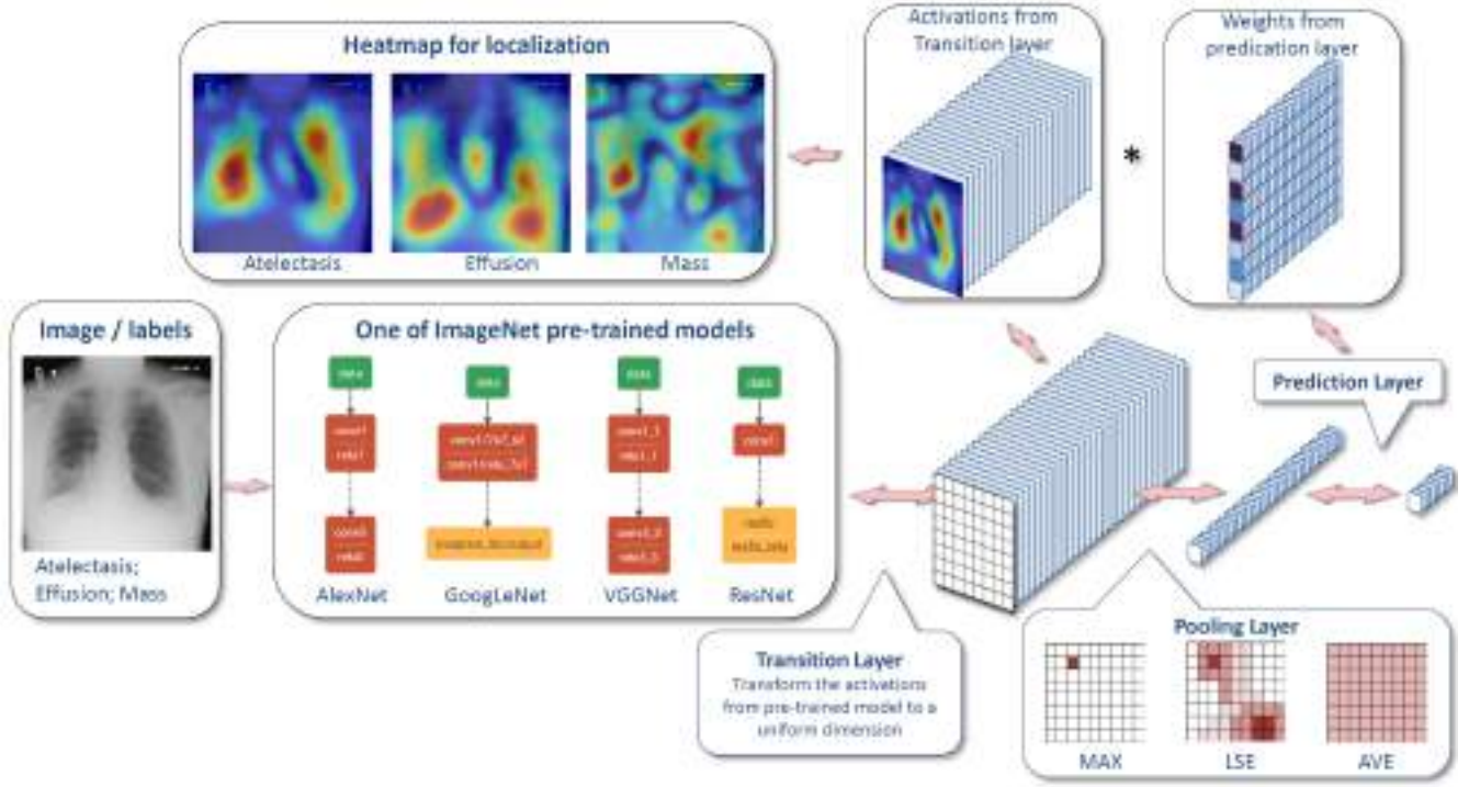
Figure 4. The overall flow-chart of our unified DCNN framework and disease localization process.
