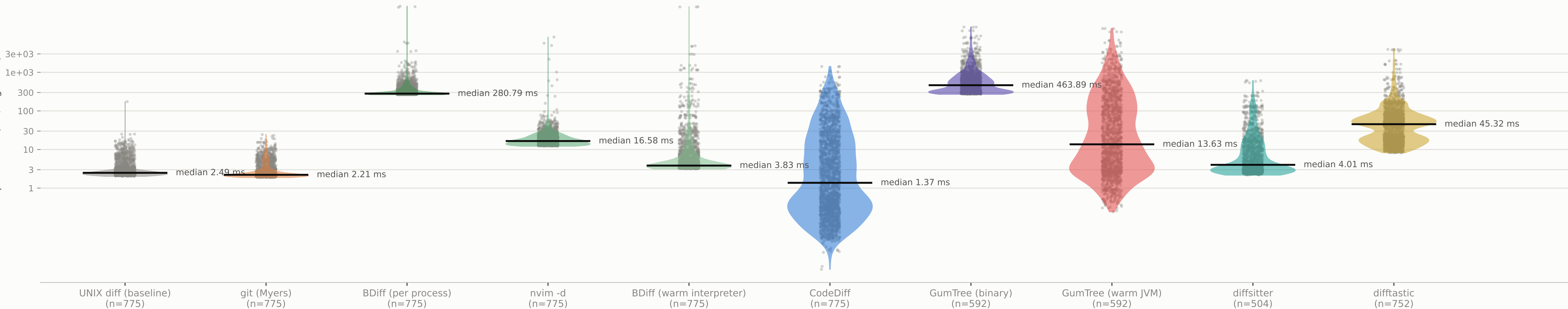
Runtime distribution: time to produce per-line touched/untouched labels (sample size varies by tool, see x-axis)
