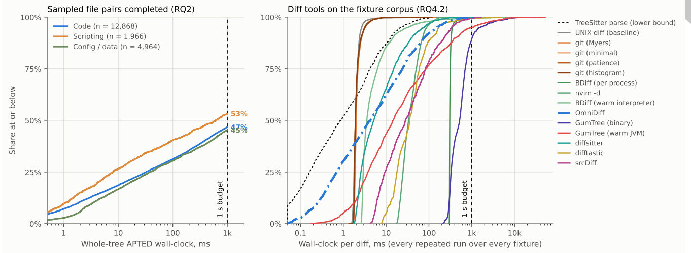
Figure 4: The one-second budget, read the same way twice. Left: the share of sampled file pairs whose whole-tree APTED computation completes within the time on the axis, per artifact category; the height of each curve at the dashed line is RA2, and the pairs the budget killed are the gap to 100%. Right: wall-clock per diff for every tool configuration of Section 7, every repeated run over every fixture, with OmniDiff charged for its parse and drawn dash-dotted; the dotted curve is the tree-sitter parse alone, the floor every AST-aware tool pays first. The dashed line is the same one second in both panels.
