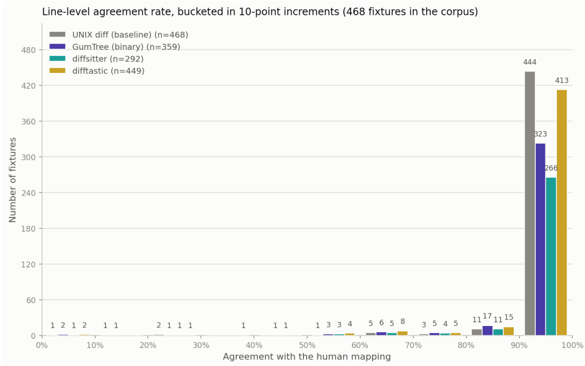
Figure 3: Line-level agreement rate with the human mapping, bucketed in 10-point increments, all four tools on the same axis. Each series’ own n reflects its applicable subset of the corpus.
