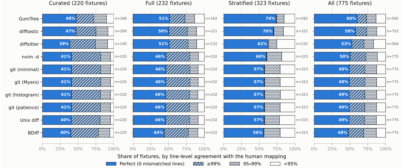
Figure 5: The line-level agreement of Table 4, split by the dataset of Section 3 each fixture was drawn from, with the pooled reading on the right. Each bar is one configuration over the fixtures it supports ( n beside the bar); the segments are the four agreement buckets, and the Perfect segment carries its share.
