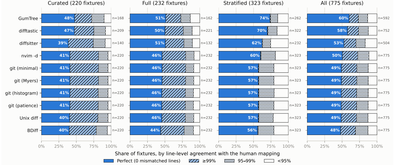
Figure 5: The line-level agreement of Table 3, split by the dataset of Section 3 each fixture was drawn from, with the pooled reading on the right. Each bar is one configuration over the fixtures it supports ( n beside the bar); the segments are the four agreement buckets, and the Perfect segment carries its share.
