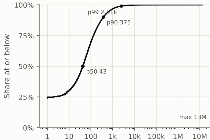
Lines per code file (n = 4,688,419)
