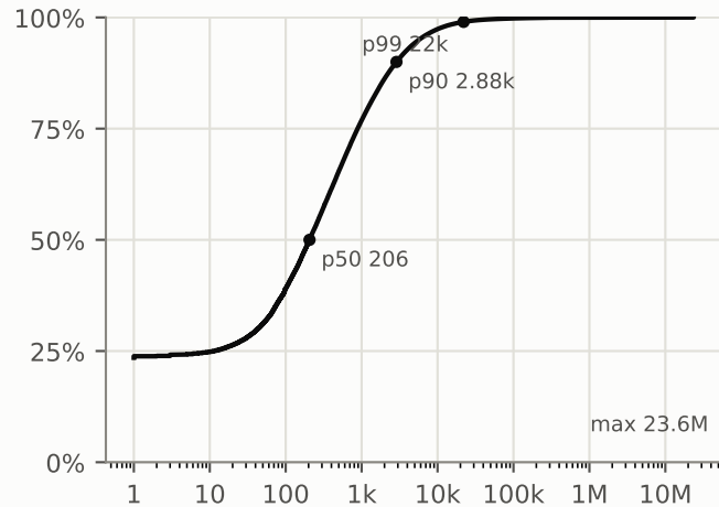
AST nodes per code file (n = 4,688,419)
