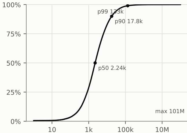
Bytes per code file (n = 4,688,419)
