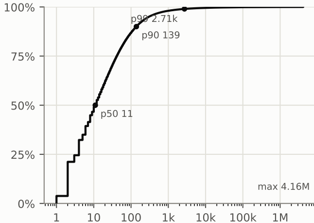
Lines changed per commit (n = 114,817)
