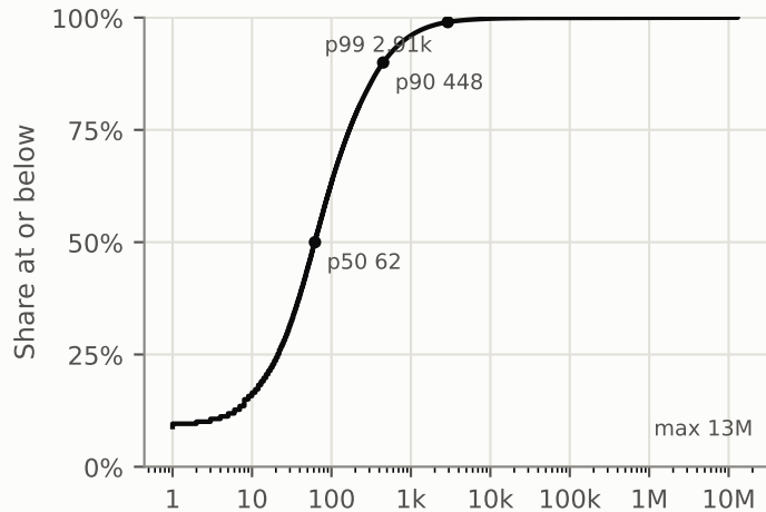
Lines per code file (n = 3,890,994)
