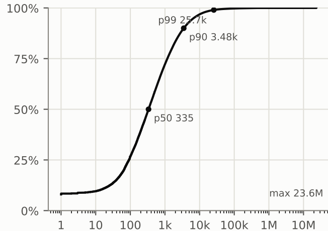
AST nodes per code file (n = 3,890,994)
