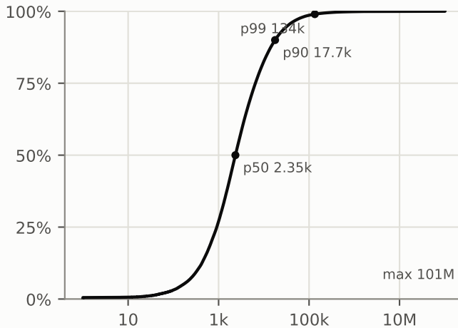
Bytes per code file (n = 3,890,994)
