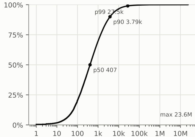
AST nodes per code file (n = 3,586,682)
