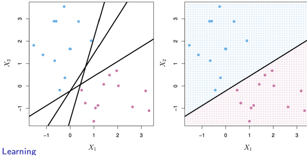
Figure 13: Different possible separating hyperplanes for linearly separable data.
