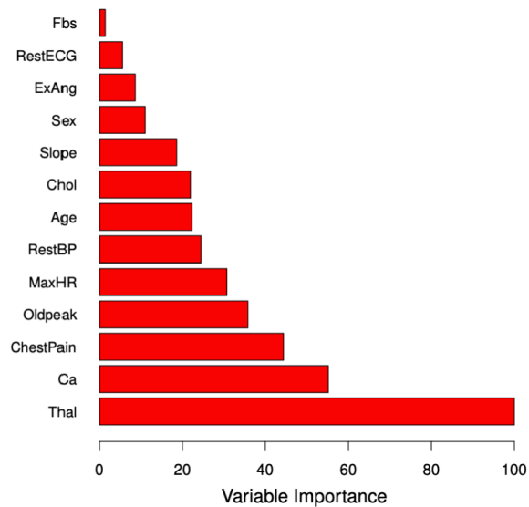
Figure 8: Variable importance in the heart disease dataset
