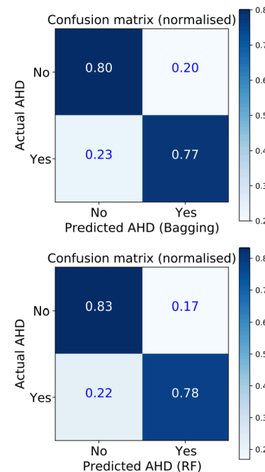
Figure 7: Confusion matrices for bagging and random forest.
