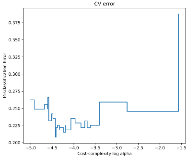
Figure 39: Cross-validation error plot
